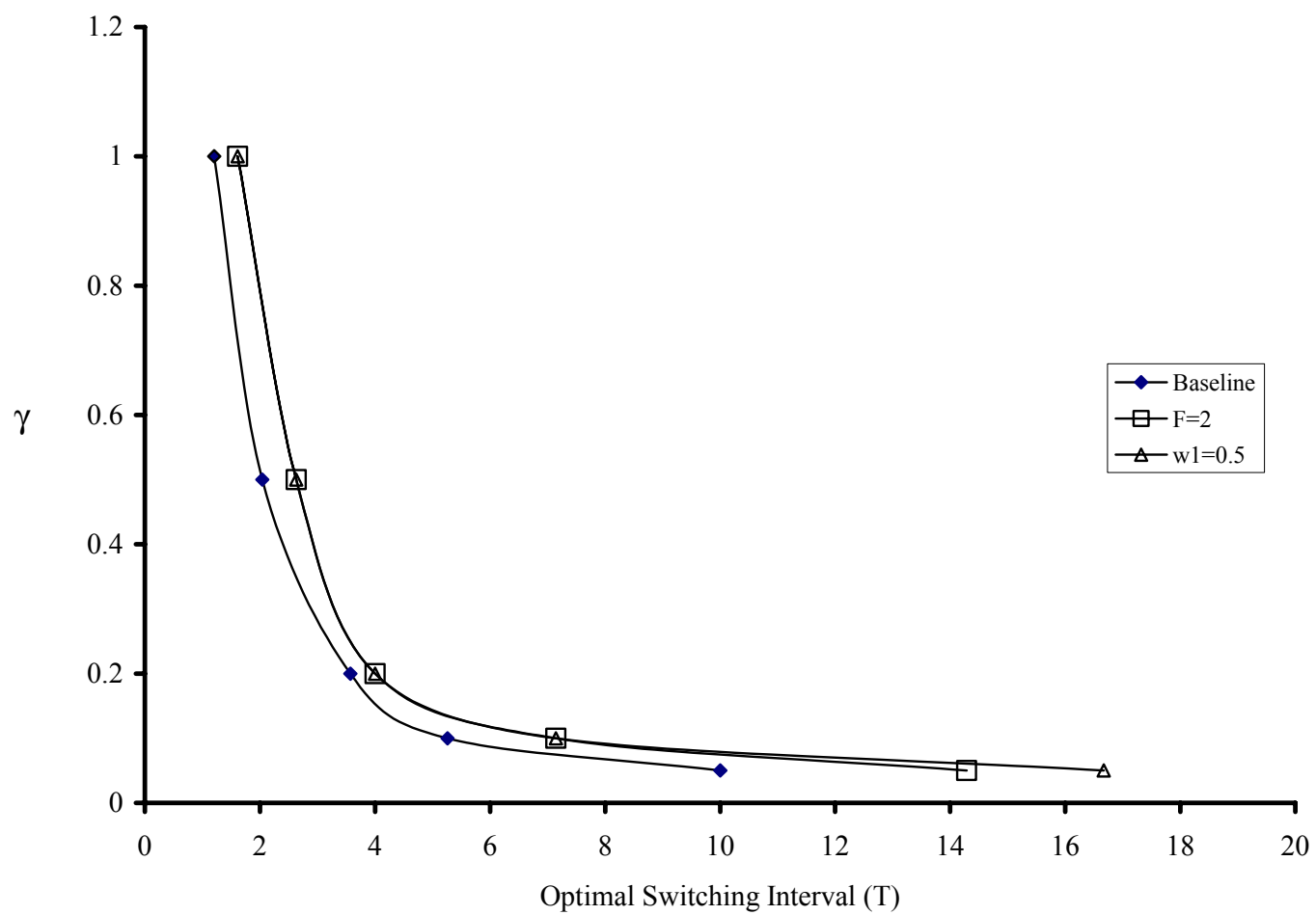
Figure 5: Sensitivity Analysis
